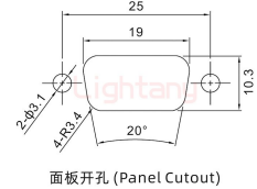
面板开孔 (Panel Cutout)
